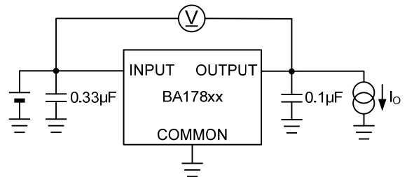
Test Circuit F. Dropout Voltage vs Output Current
