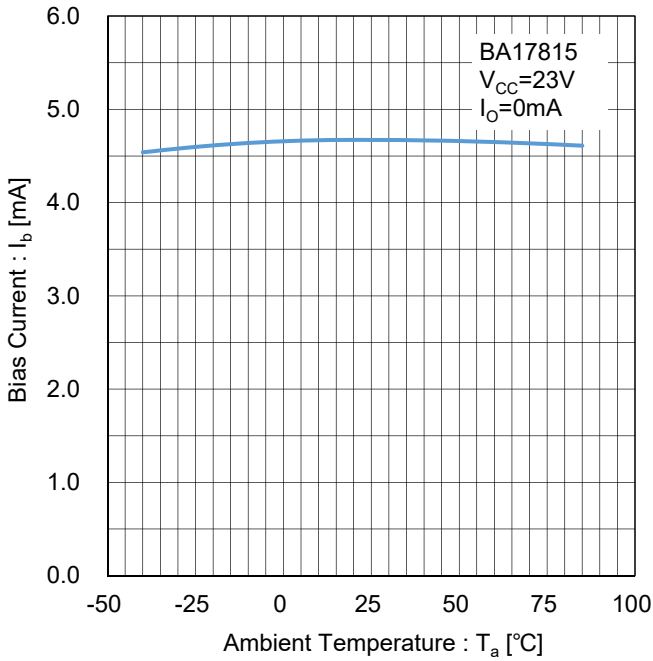
Figure 93. Bias Current vs Temperature Test Circuit I
