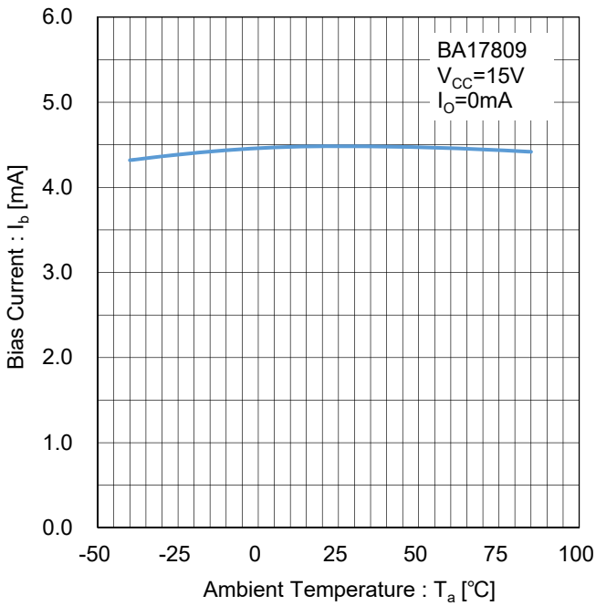
Figure 57. Bias Current vs Temperature Test Circuit I
