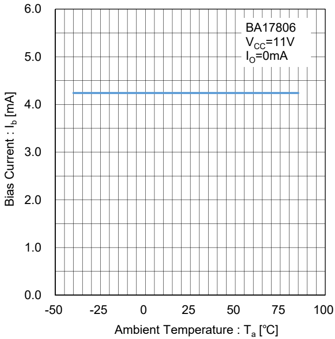
Figure 21. Bias Current vs Temperature Test Circuit I
