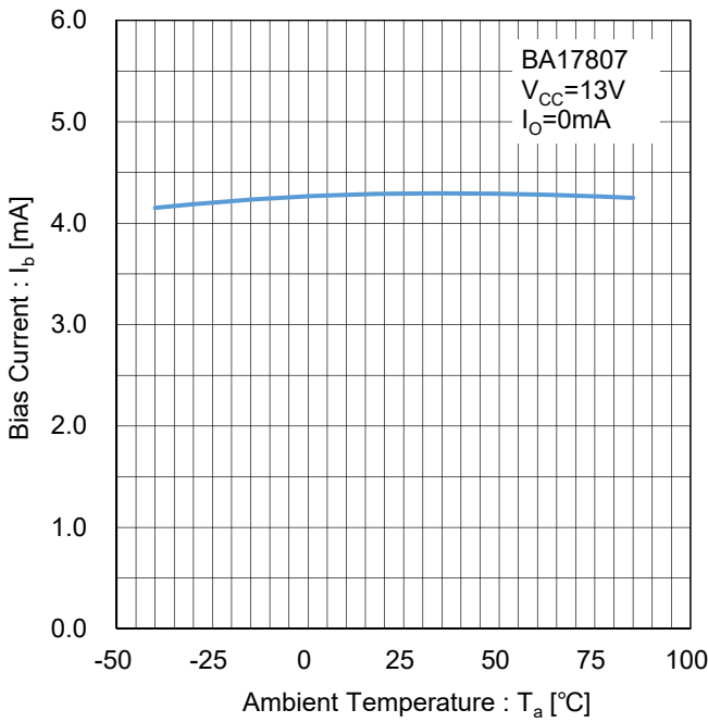
Figure 33. Bias Current vs Temperature Test Circuit I
