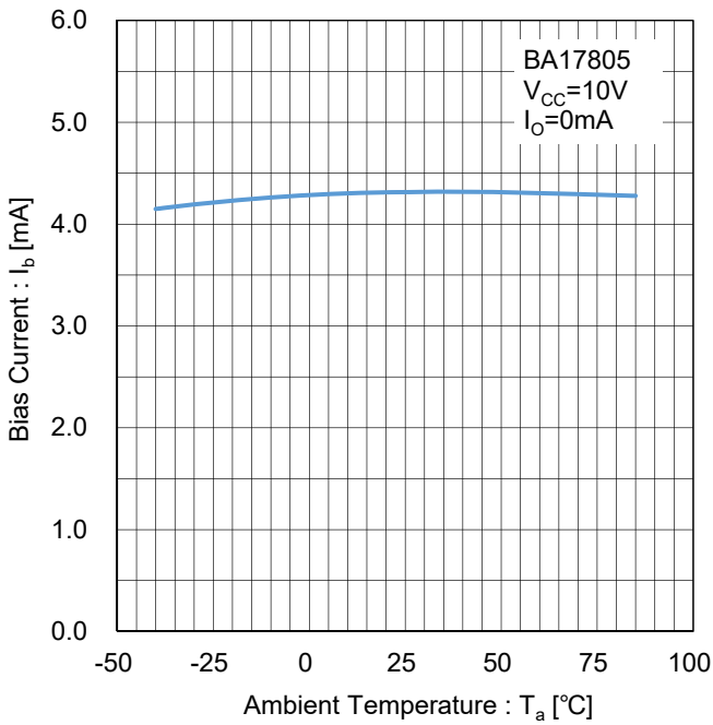
Figure 9. Bias Current vs Temperature Test Circuit I
