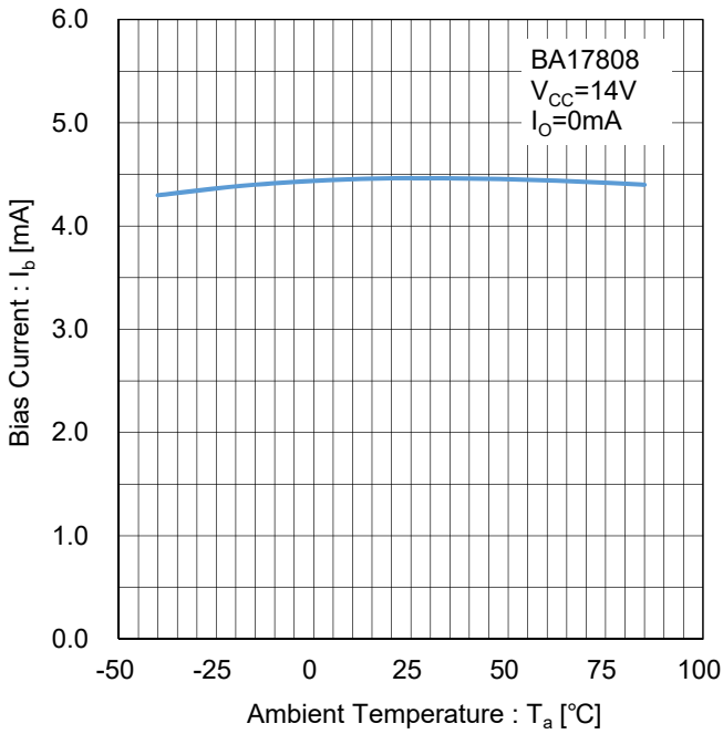
Figure 45. Bias Current vs Temperature Test Circuit I
