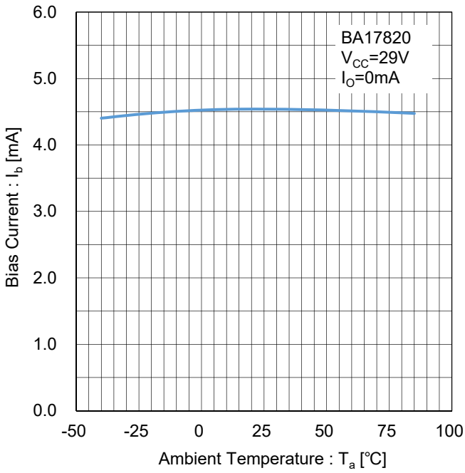
Figure 117. Bias Current vs Temperature Test Circuit I
