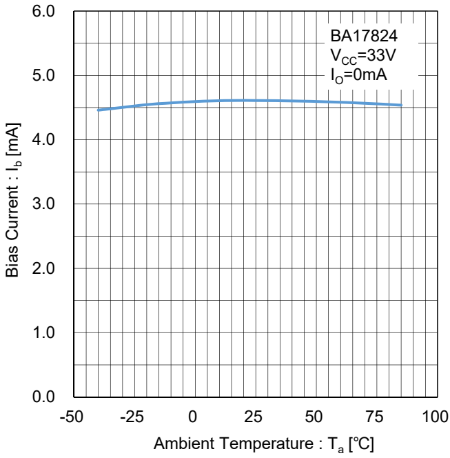
Figure 129. Bias Current vs Temperature Test Circuit I
