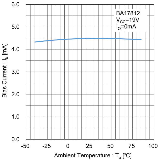
Figure 81. Bias Current vs Temperature Test Circuit I
